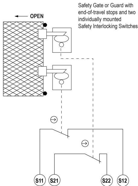
Figure 3. Wiring using contacts from two safety switches
