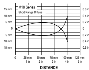
Beam Pattern
