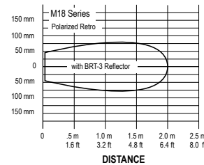
Beam Pattern
