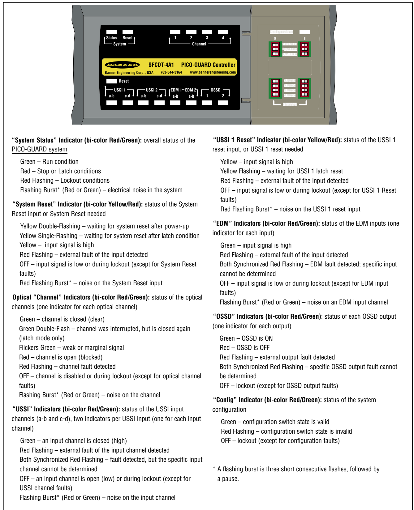
Figure 4-3. PICO-GUARD controller status indicators
