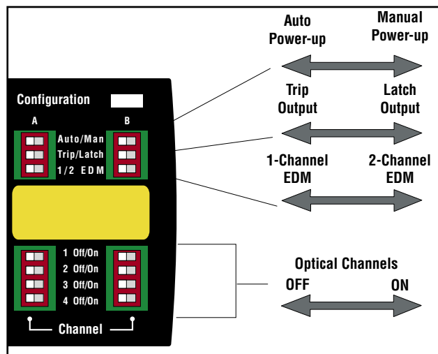
Figure 3-6. Configuration DIP switches
