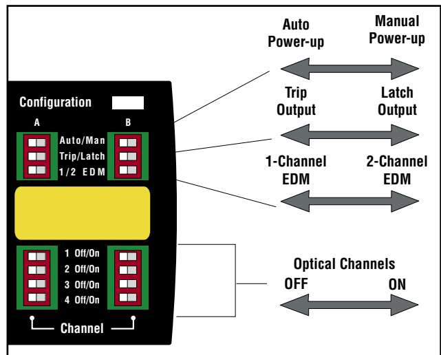
Figure 4-2. PICO-GUARD controller configuration switches
