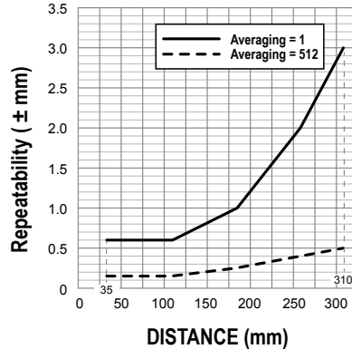
Figure 28. 310 mm Models
